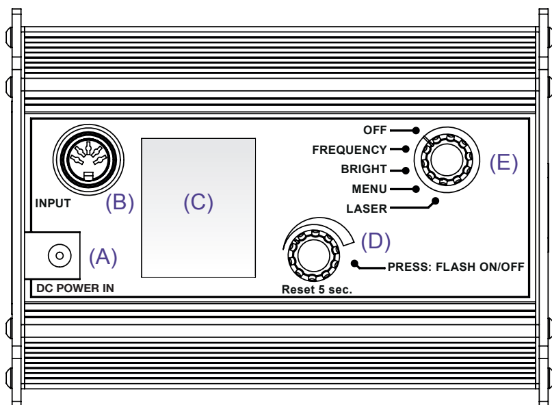
Fig.1 - Stroboscope LS-3-LED
