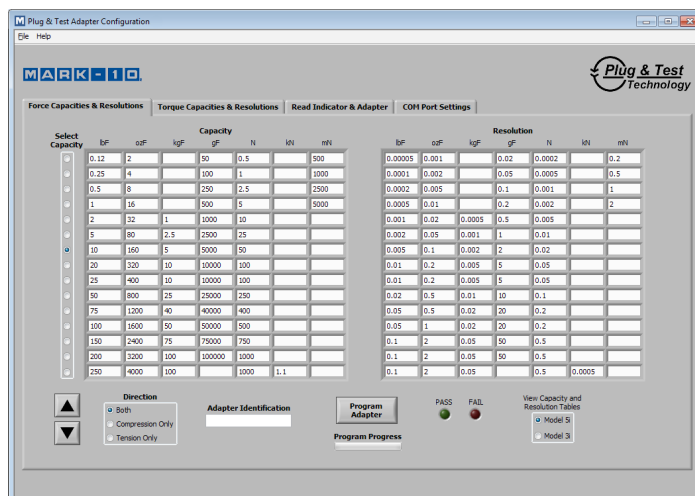
^ Software utility features a library of force and torque capacities. Programming of capacity, resolution, and identification number is done via USB through the 5i or 3i indicator.
